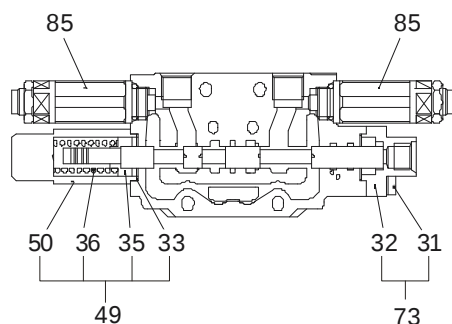
"I-I"SECTION
