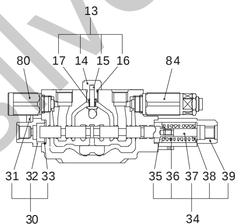
"M-M"SECTION
