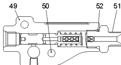
"E-E" SECTION
