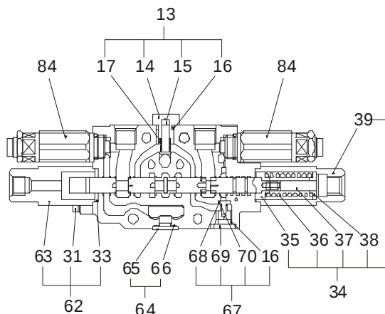
"G-G"SECTION
