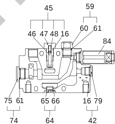
"L-L"SECTION
