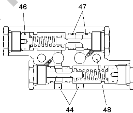
"D-D" SECTION
