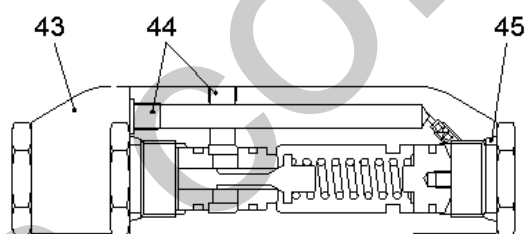
"C-C" SECTION
