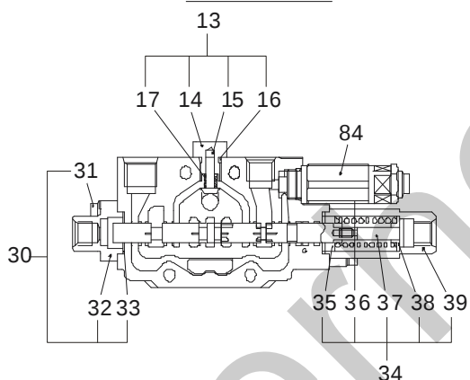
"K-K"SECTION
