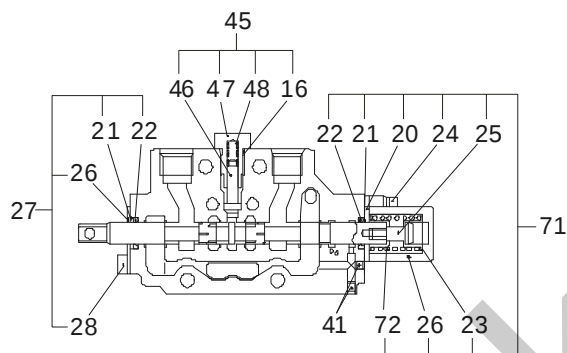
"H-H"SECTION
