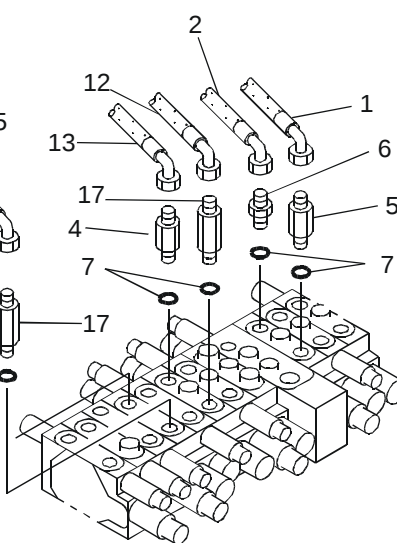
"D" DETAIL
