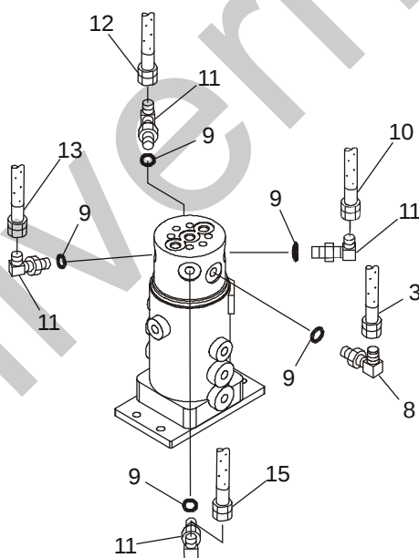
"C" DETAIL
