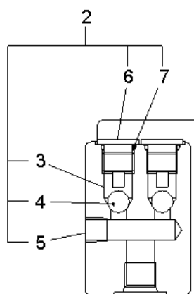
"A-A" SECTION
